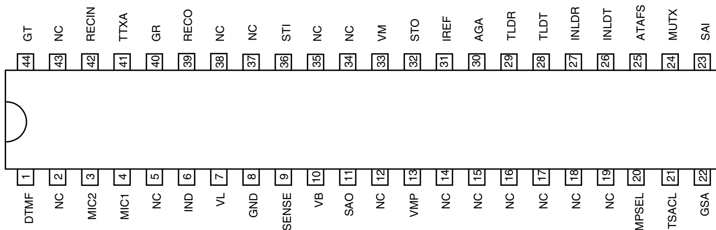
Figure 2-1. Pinning SSO44
