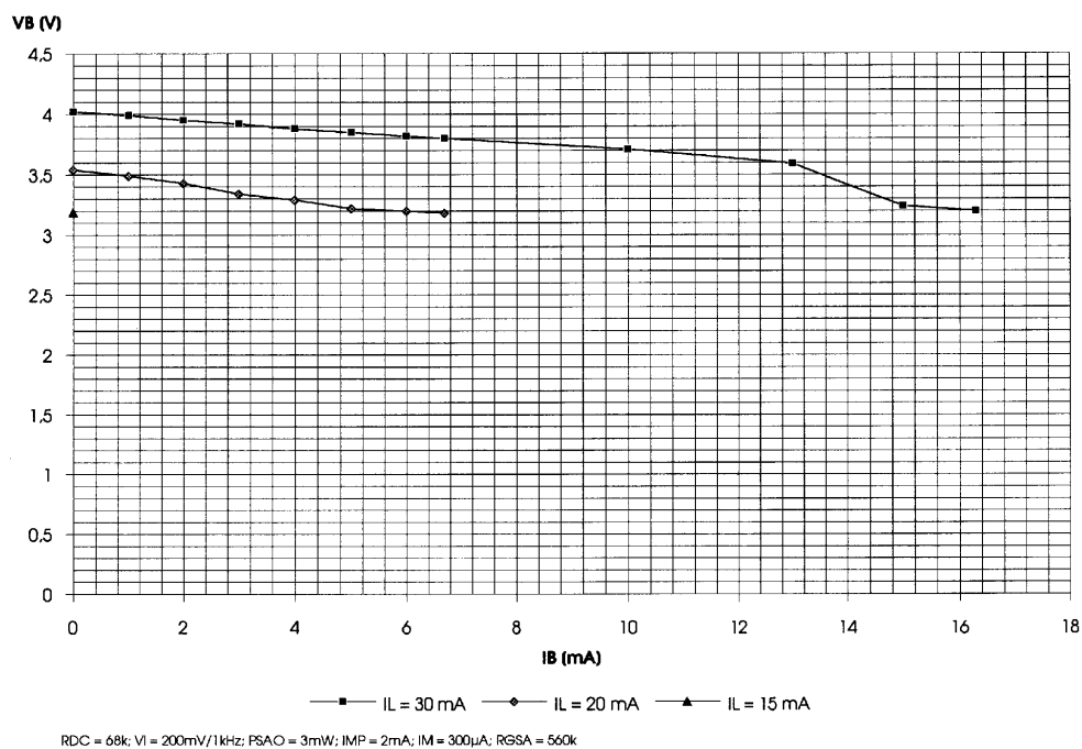
Figure 8-7. Typical Load Characteristic of V_B for a Minimum DC Characteristic ( R_{DC} = 68k\Omega ) and a 3-mW Loudspeaker Output
